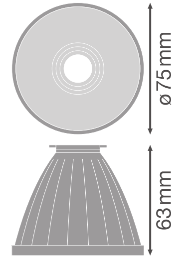
TRACK SP REFLECTOR D85 SP
