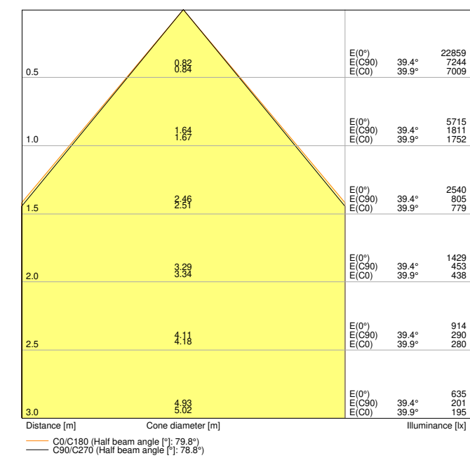
LEDV LOWBAY 100W 850 WD 90
