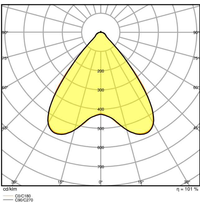
LEDV LOWBAY 100W 850 WD 90
