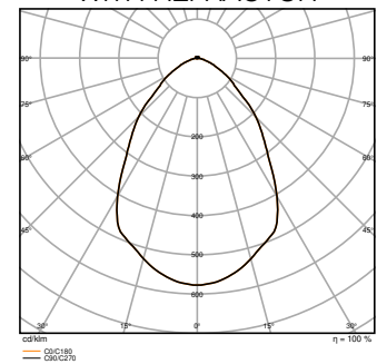
HB DA P 150W 865 110DEG IP66 WITH REFRACTOR
