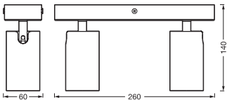
LED SPOT OCTAGON 2X3.4W 927 GU10
