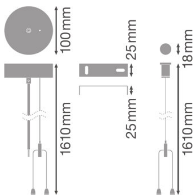
LN INDV DALI Suspension Kit
