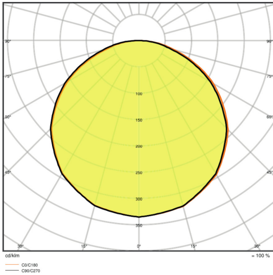
LS VAL -1400/840/5
