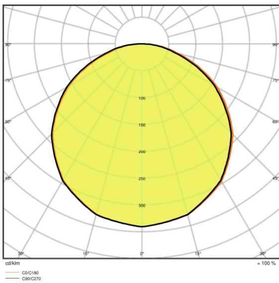
LS VAL -1400/827/5
