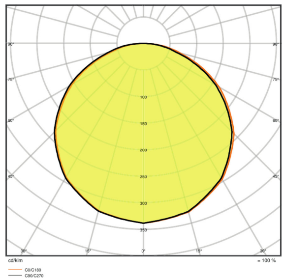
LS VAL -1400/830/5
